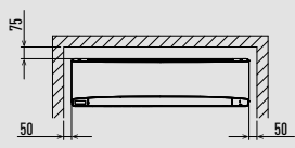
Minimum space requirements for installation
